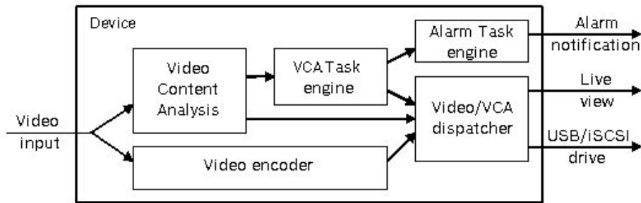
Figure 3.1 Device architecture
